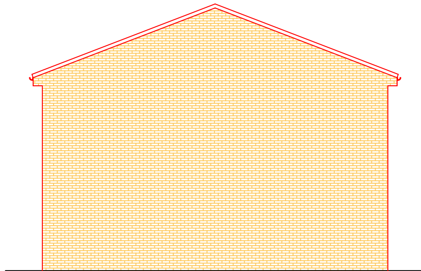
Proposed New House Side Elevation - A
