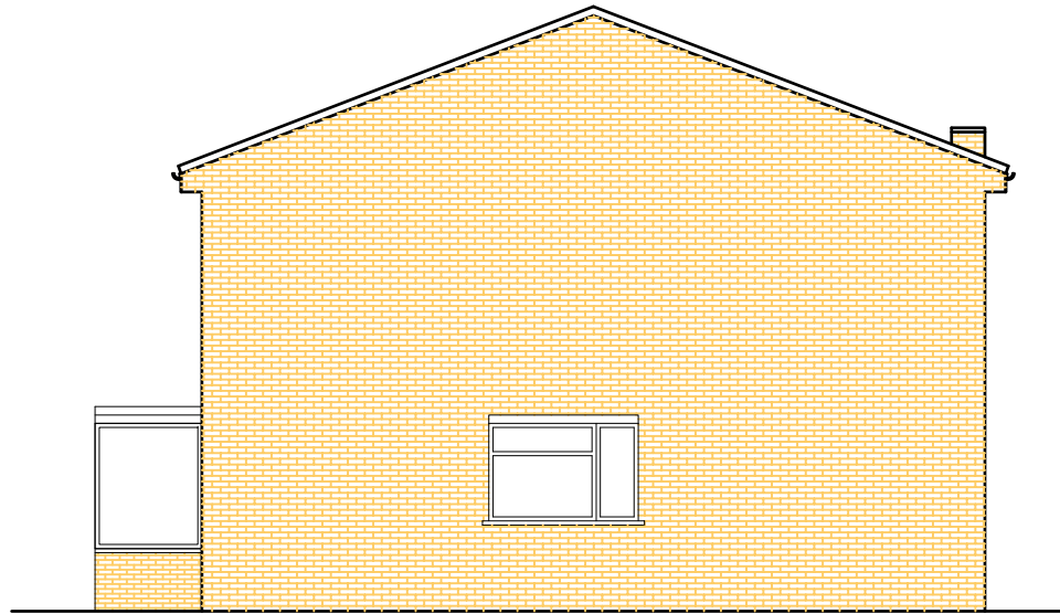
Existing Side Elevation - A
