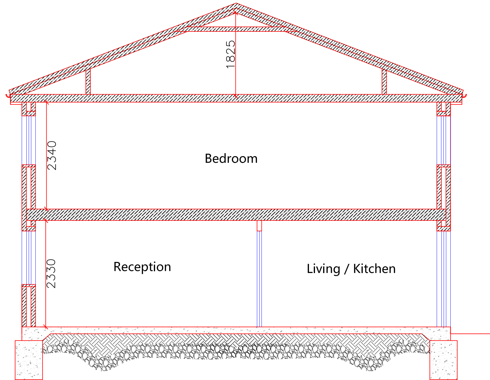
Section X-X
