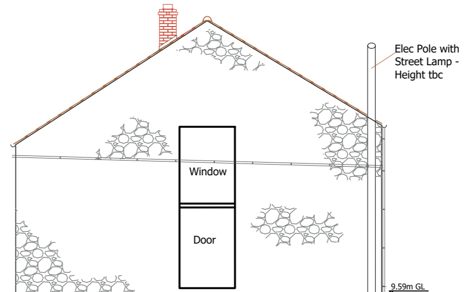
No. 21 Road Side Elevation (north) Scale 1:100
