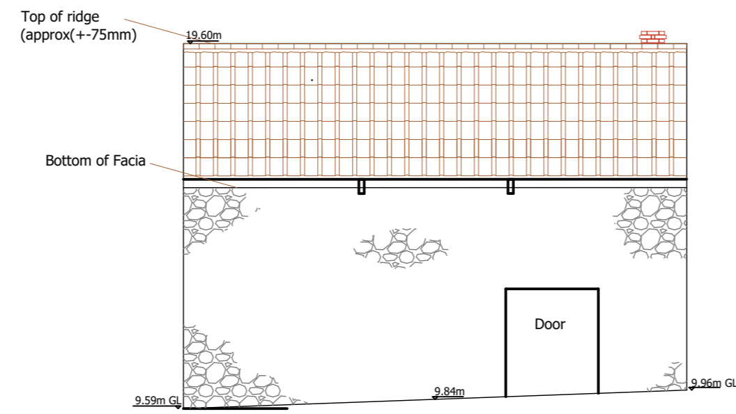
No. 21 Front Elevation (west) Scale 1:100
