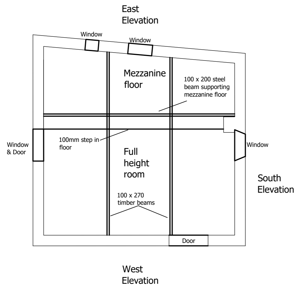
No. 21 Floor Plan with Main Beams Scale 1:100
