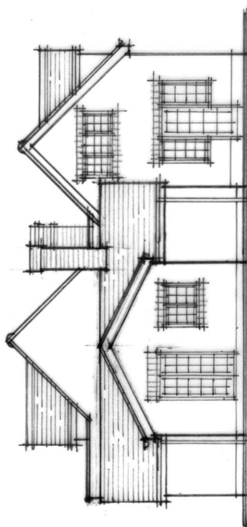
rear elevation
