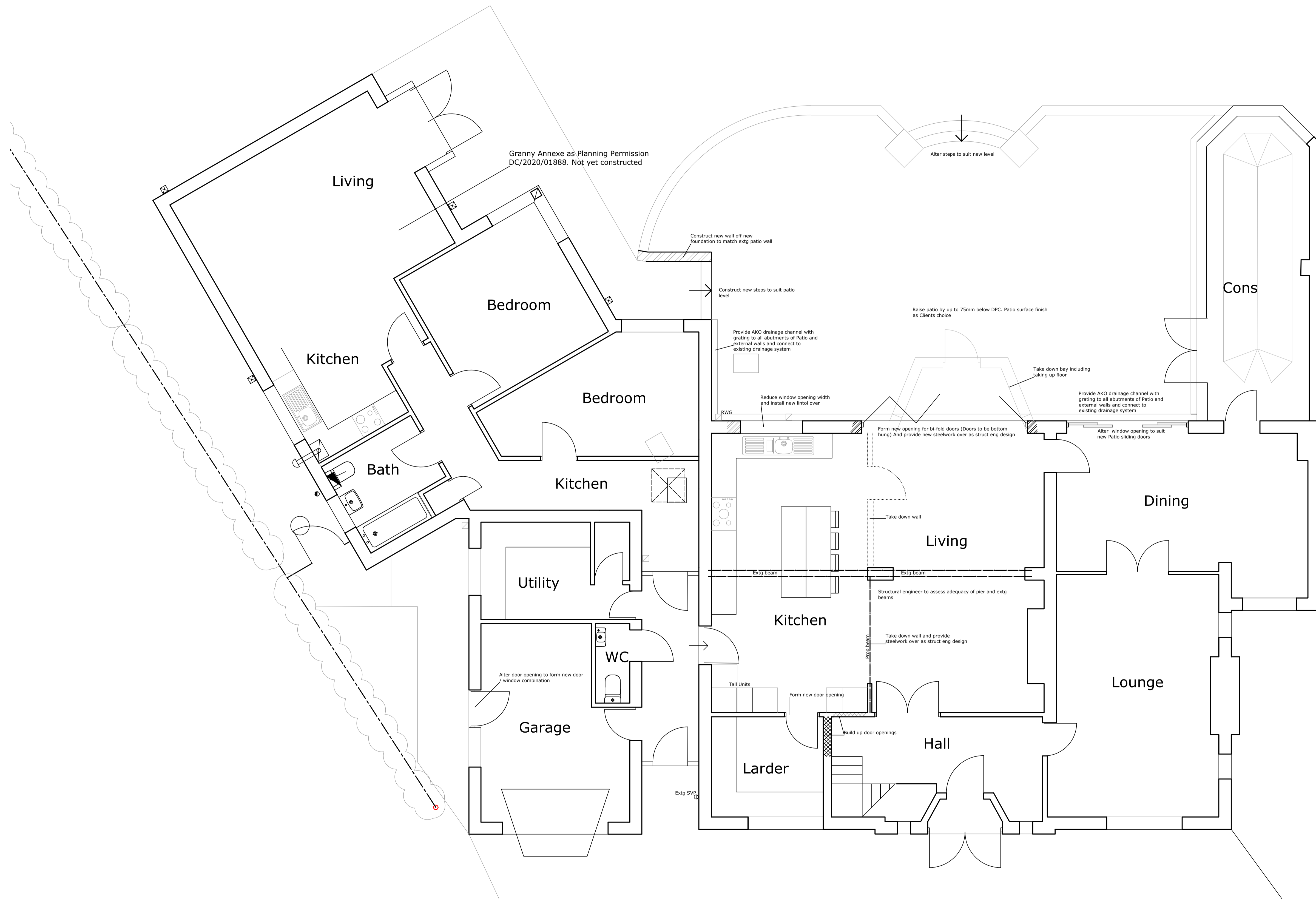
Ground Floor Plan scale 1:50
