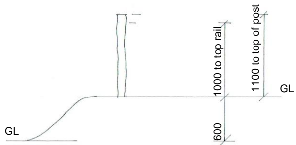
Section through fence
