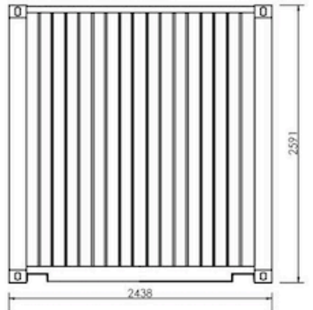
20ft Shipping Container - Front Elevation
