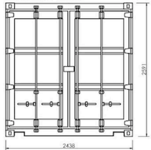
20ft Shipping Container - Door Elevation
