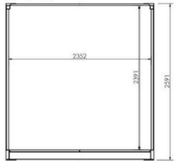
20ft Shipping Container - Section
