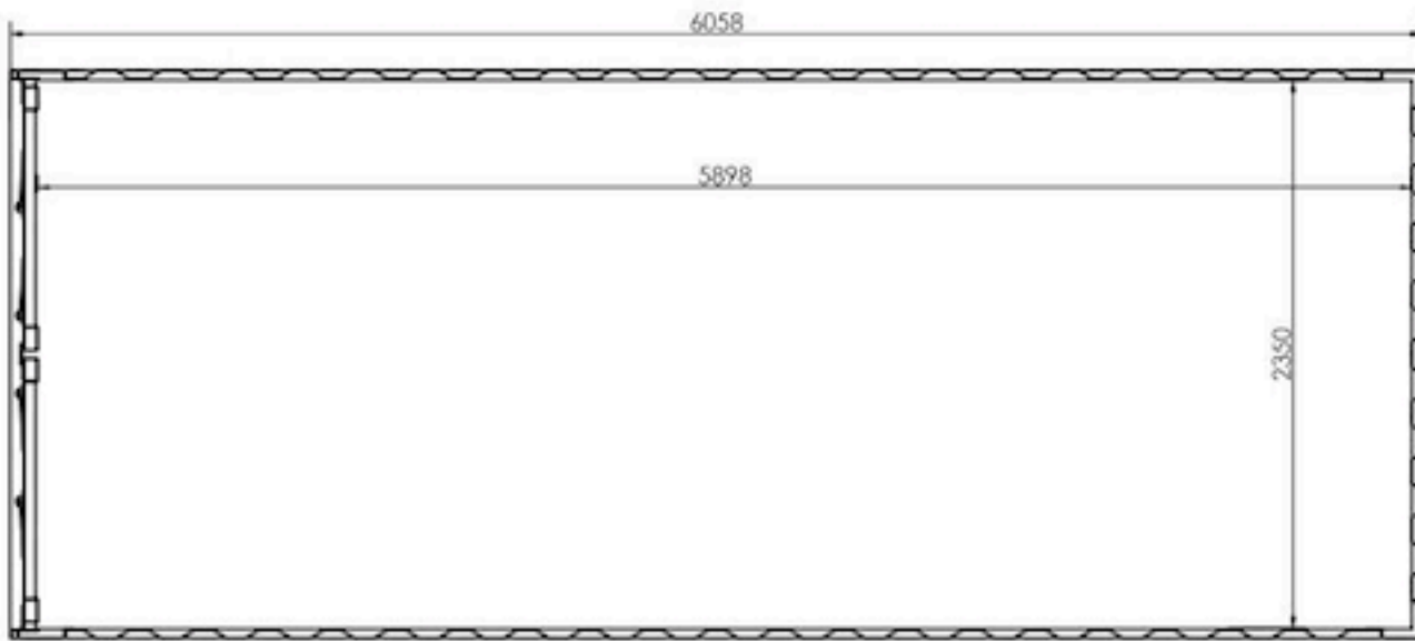
20ft Shipping Container - Plan
