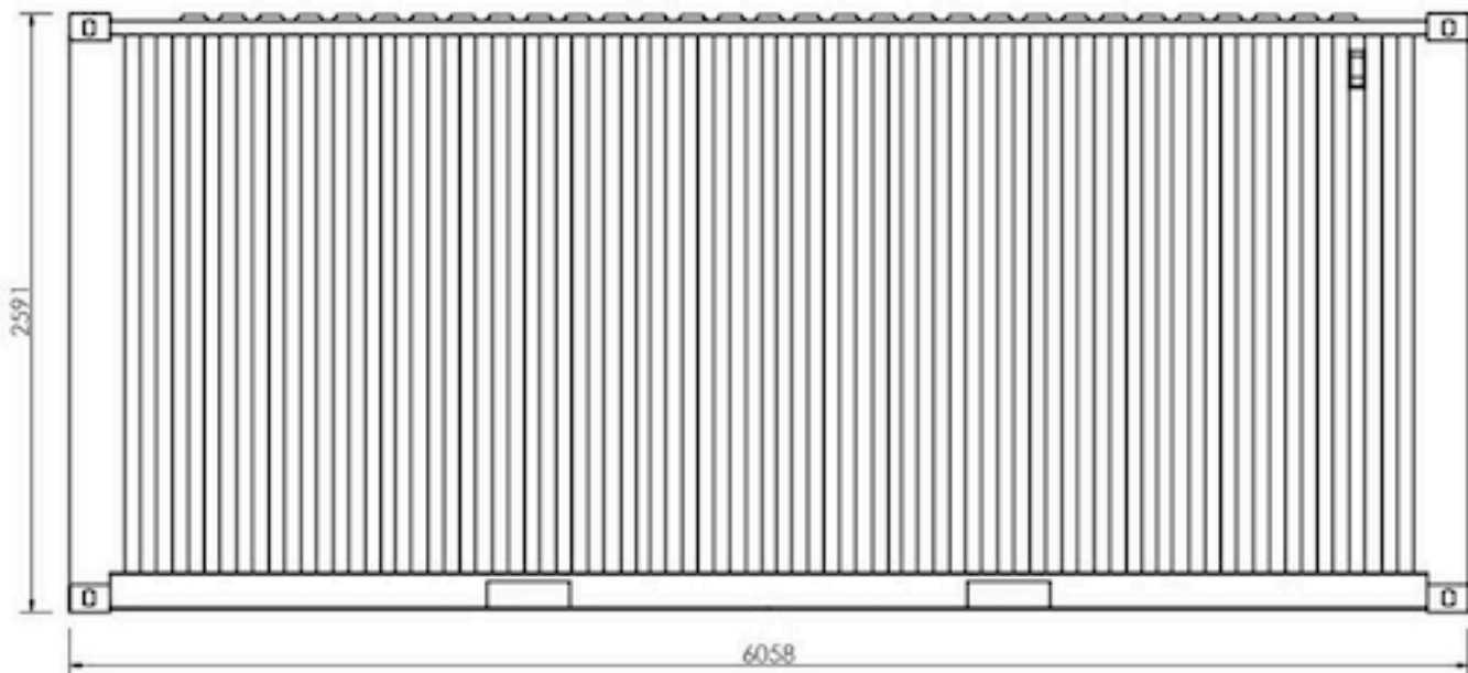
20ft Shipping Container - Side Elevation
