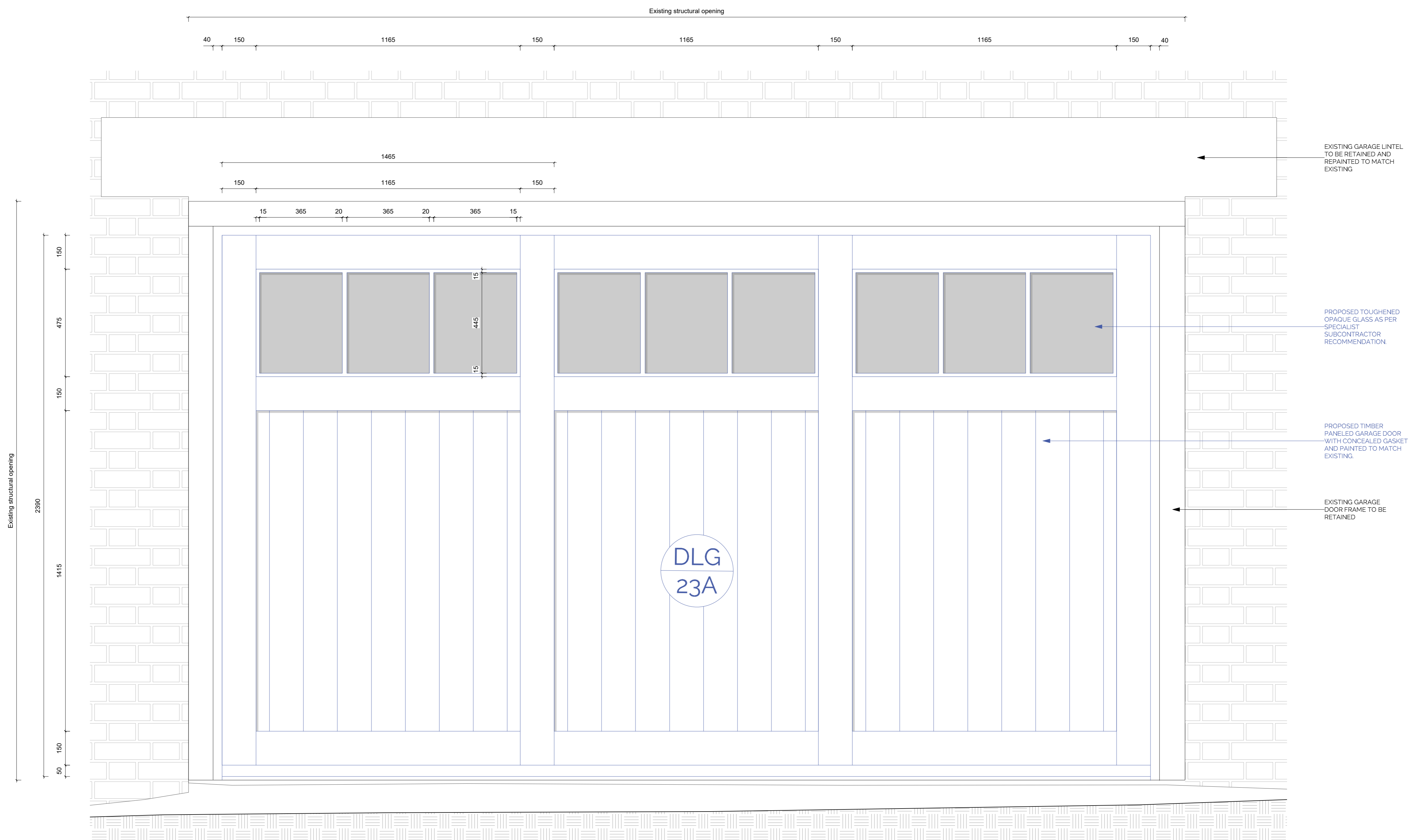
1 Proposed garage door elevation 1:10 @ A1
