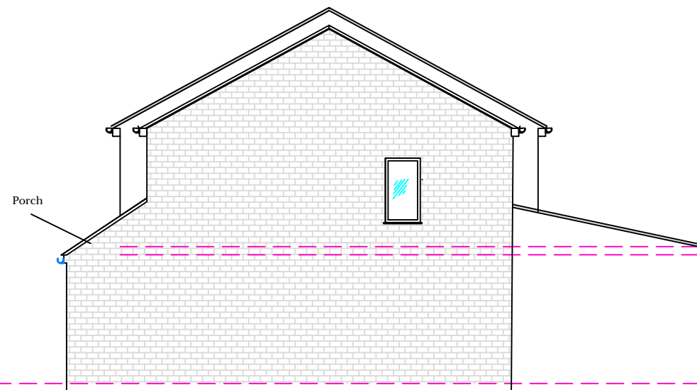
Proposed Side south
