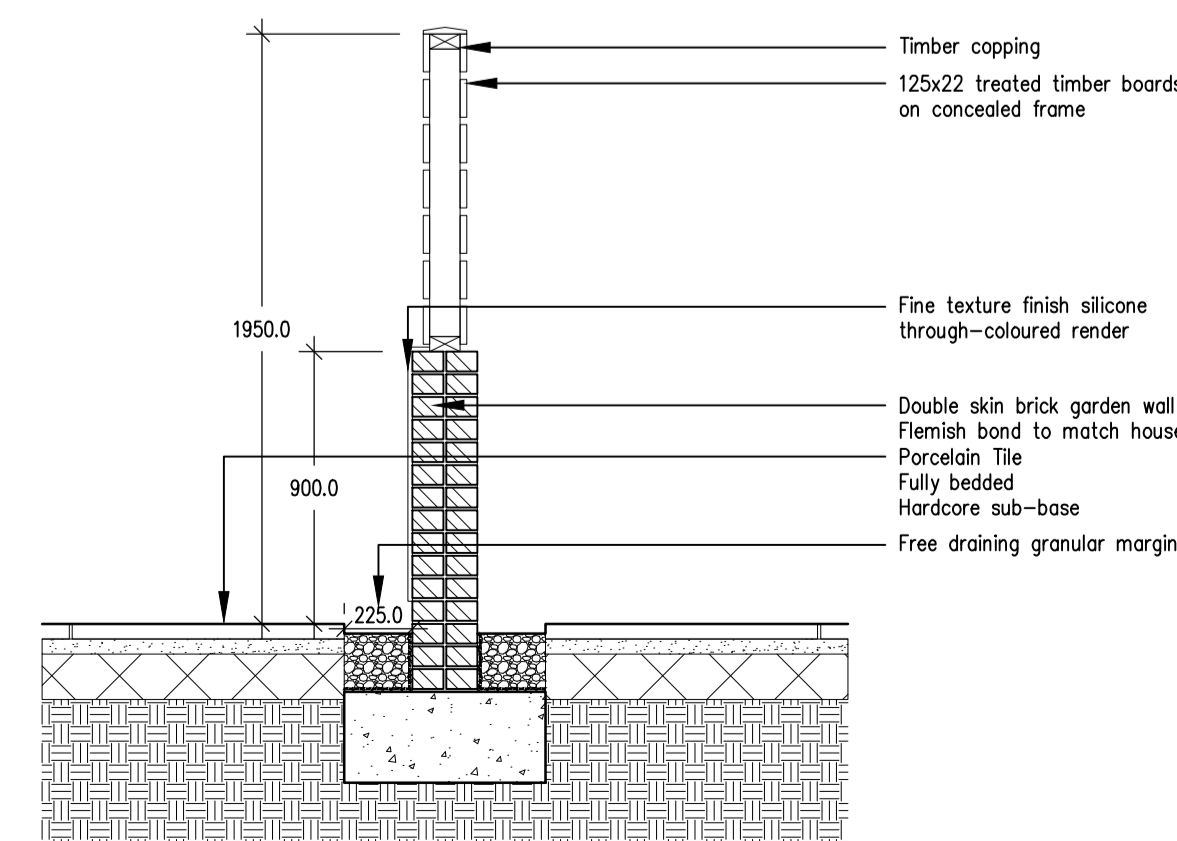
EXTERNAL WORKS DETAIL 6 (1:25)
