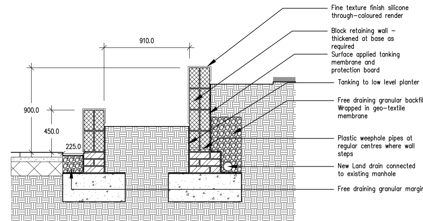
EXTERNAL WORKS DETAIL 3 (1:25)
