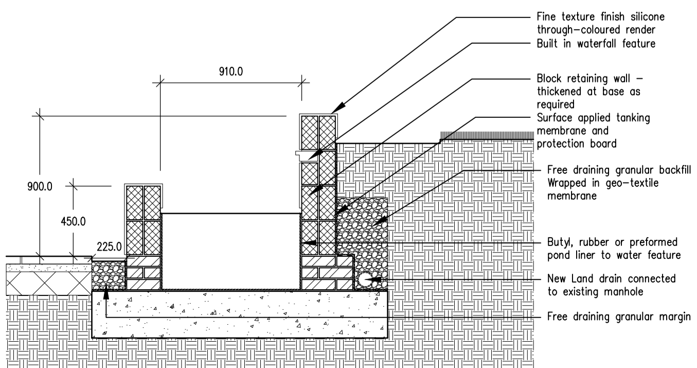
EXTERNAL WORKS DETAIL 4 (1:25)
