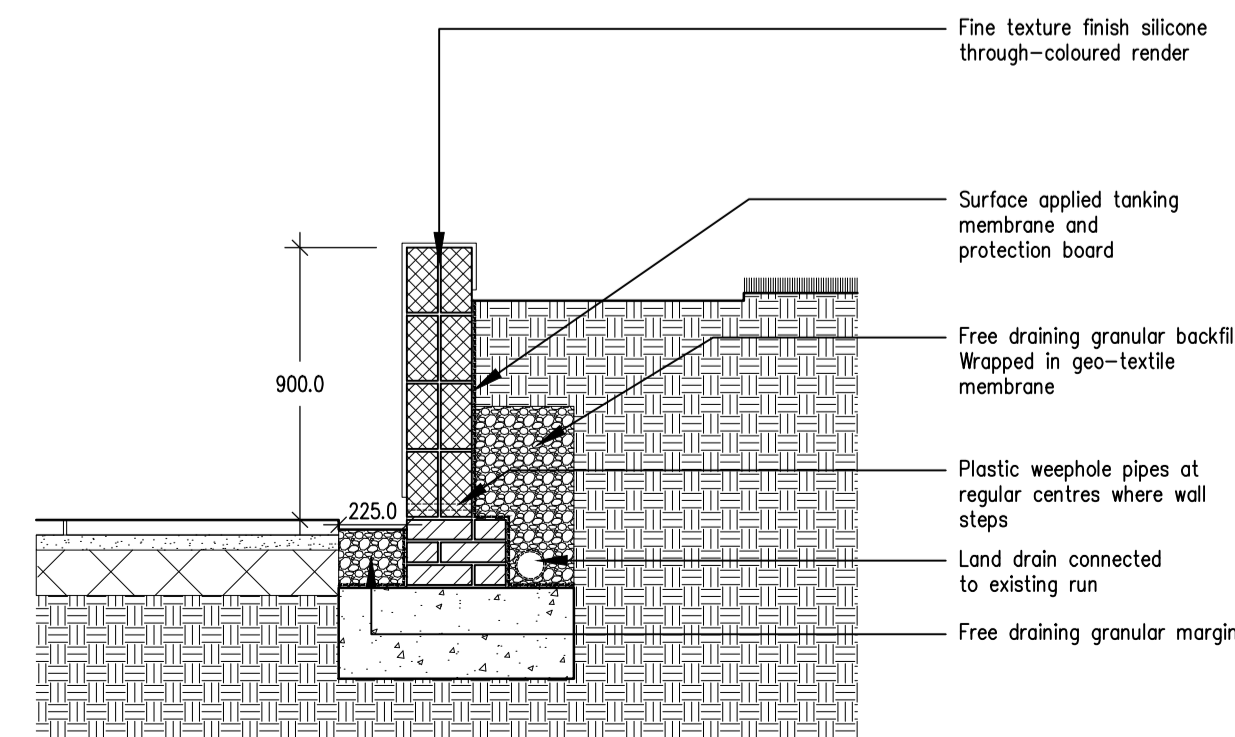
EXTERNAL WORKS DETAIL 5 (1:25)
