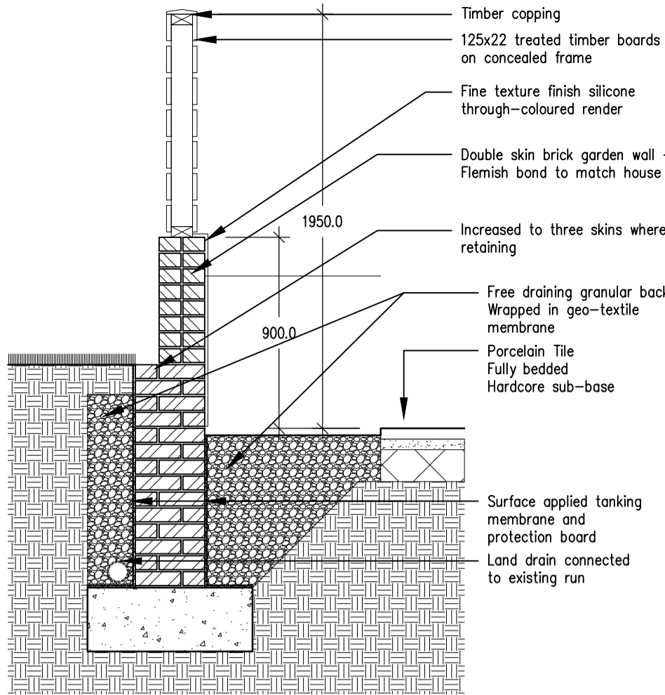
EXTERNAL WORKS DETAIL 1 (1:25)
