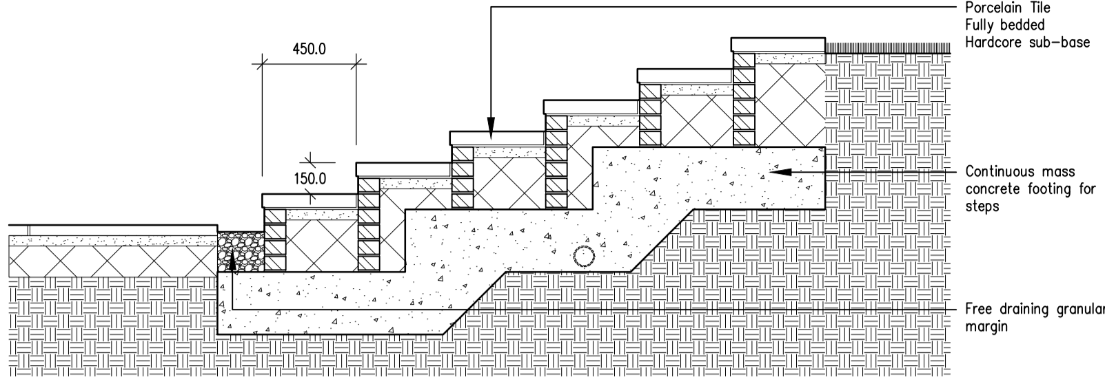
EXTERNAL WORKS DETAIL 2 (1:25)
