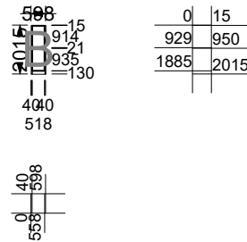
W1,W2,W3 Bottom sliding sash x 2
