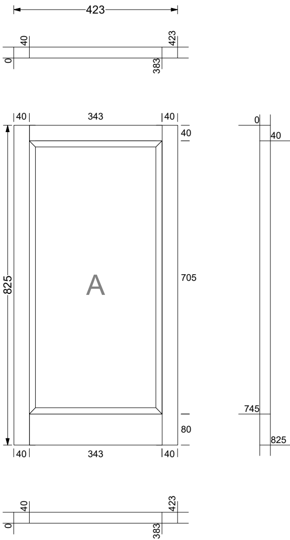
1 X Casement - W5 (Kitchen)
