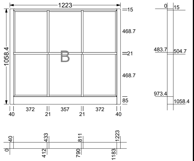
W5 Screen Casement Fixed
