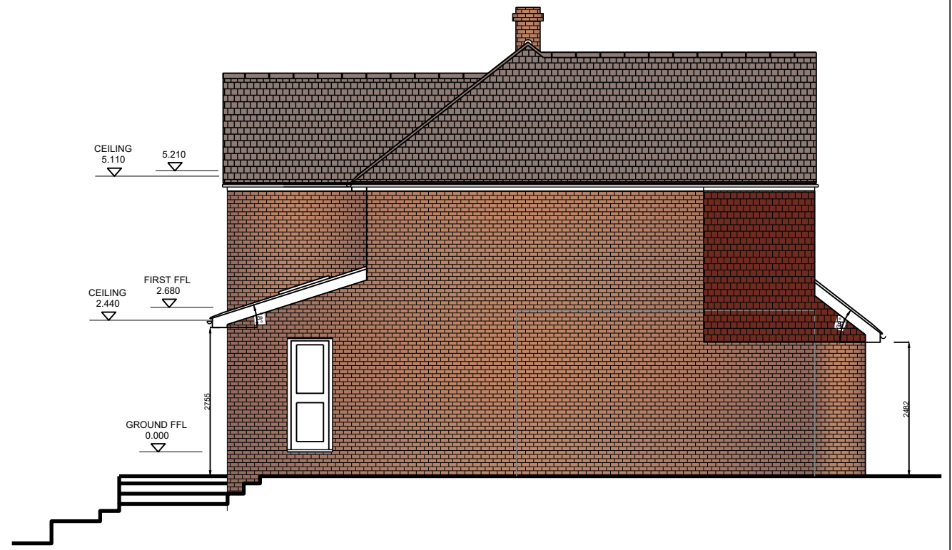
WEST ELEVATION. (1:100)
