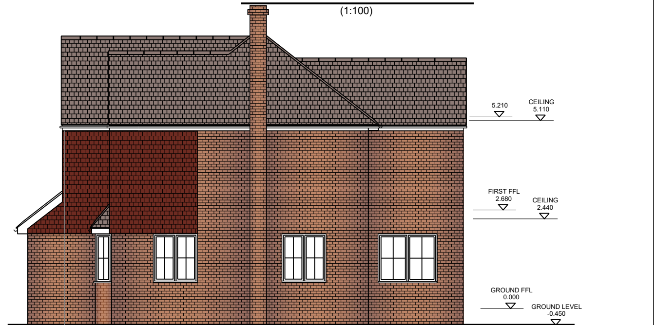
EAST ELEVATION. (1:100)
