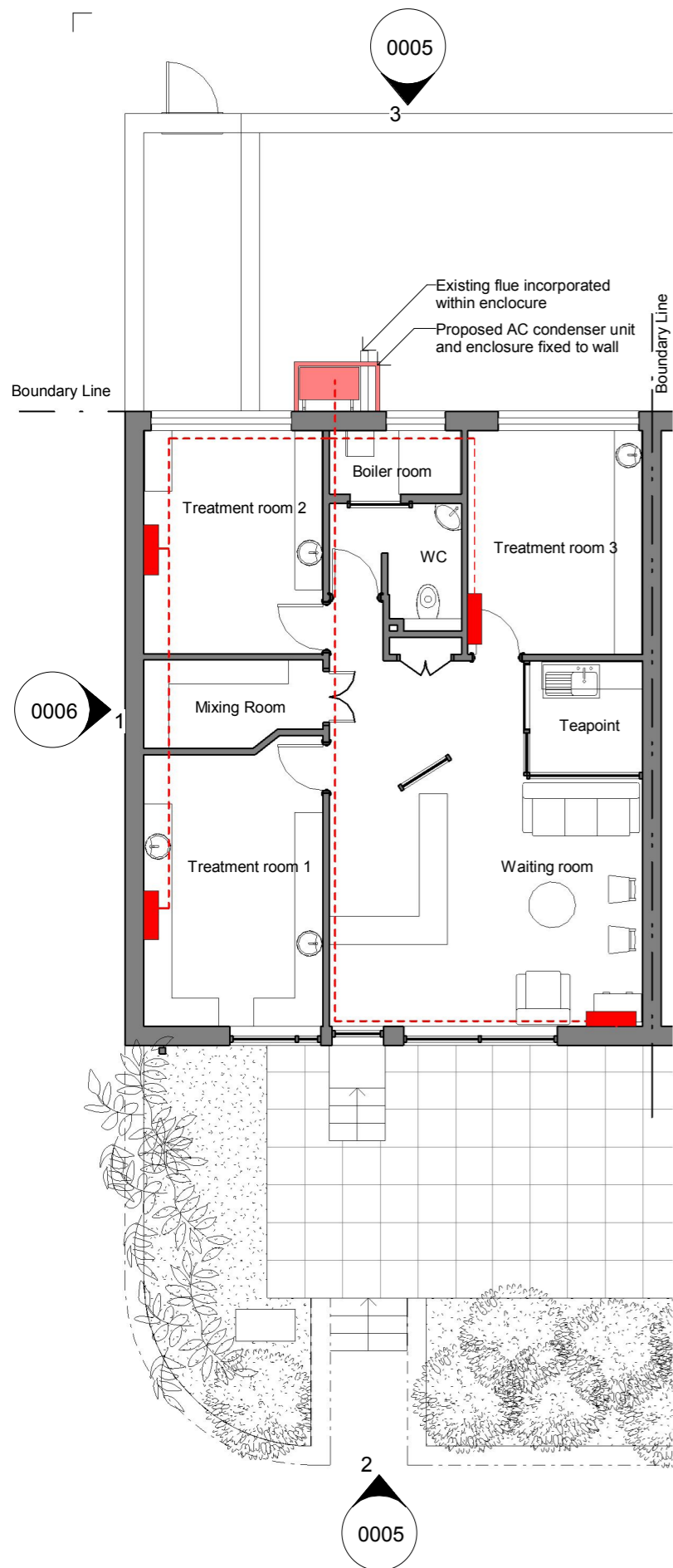
1 Proposed Ground Floor Plan 1 : 100
