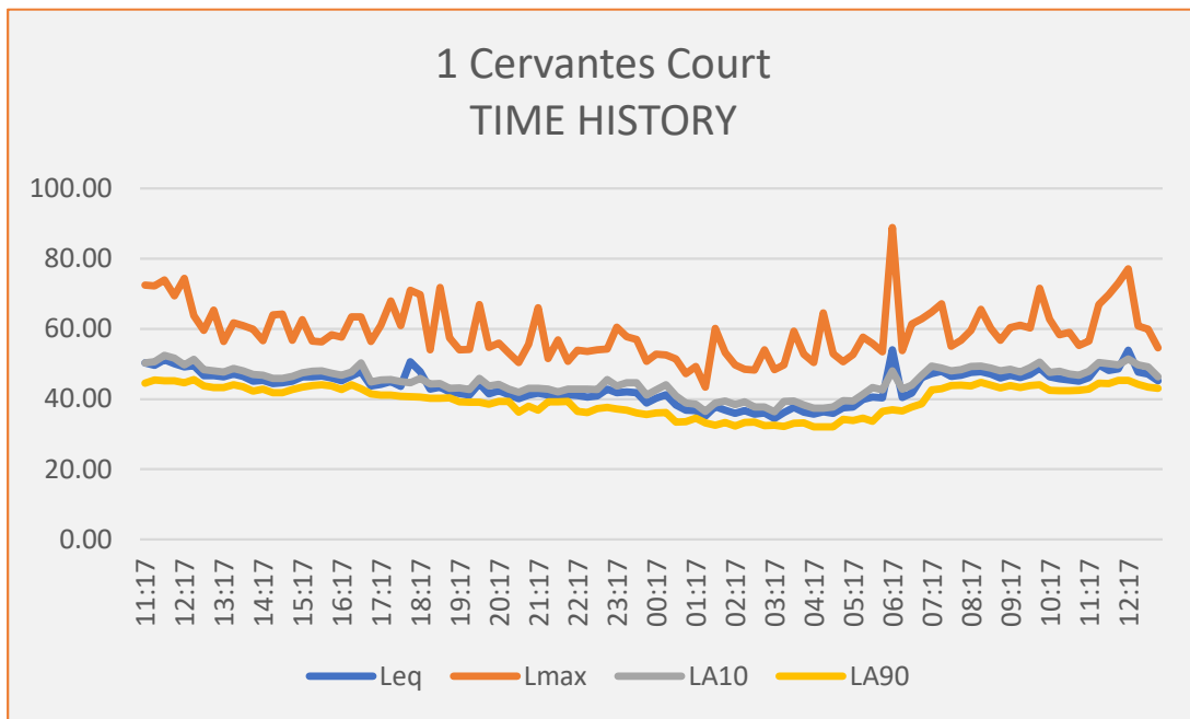
Figure 4.1.1 – Time History
