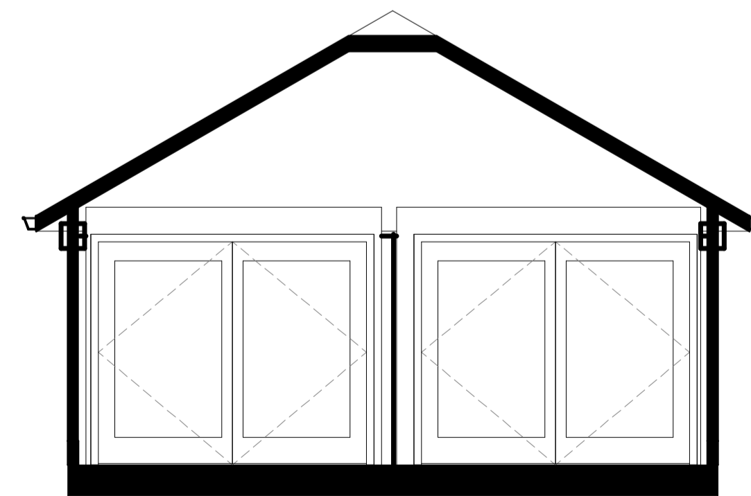
6 Typical Section 1 : 50
