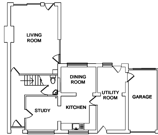
EXISTING GROUND FLOOR (1:100)
