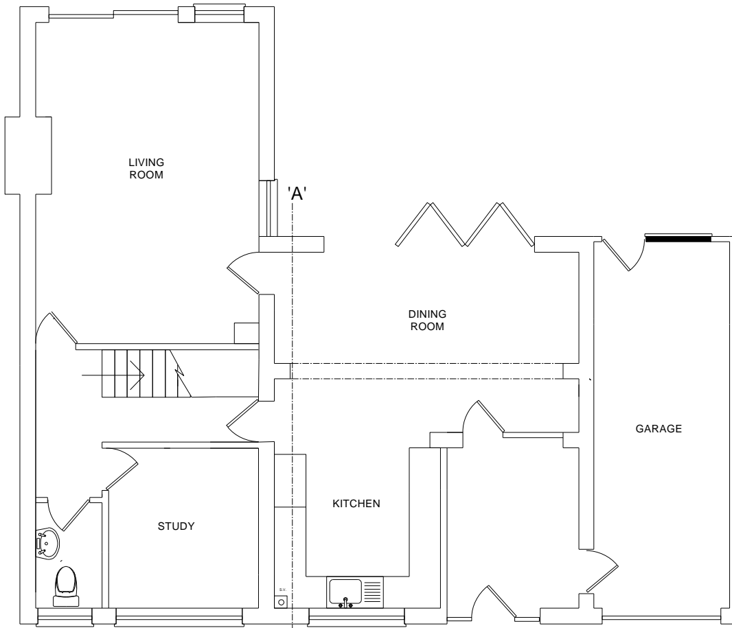
PROPOSED GROUND FLOOR PLAN (1:50)
