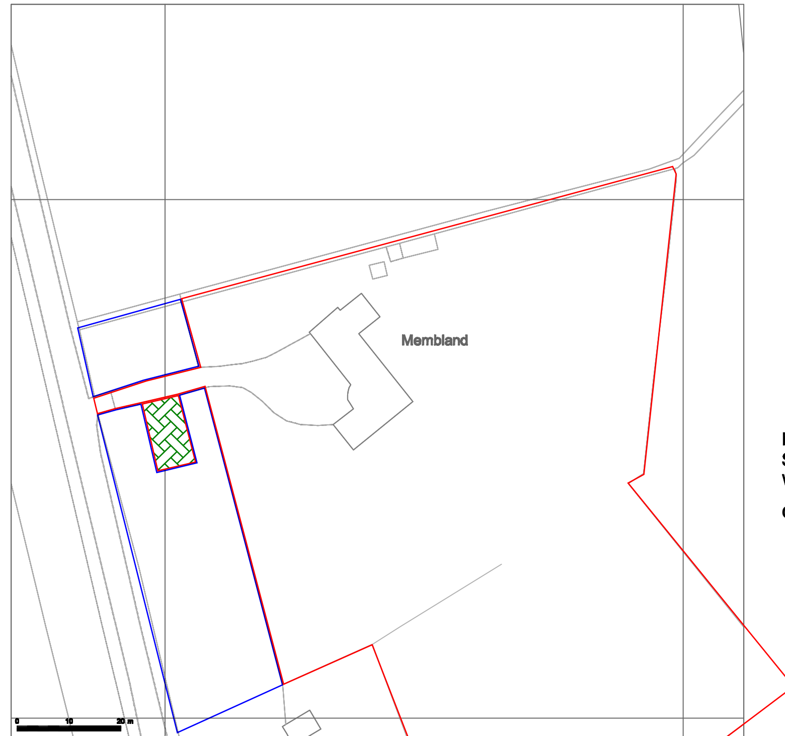
BLOCK PLAN - 1:500
