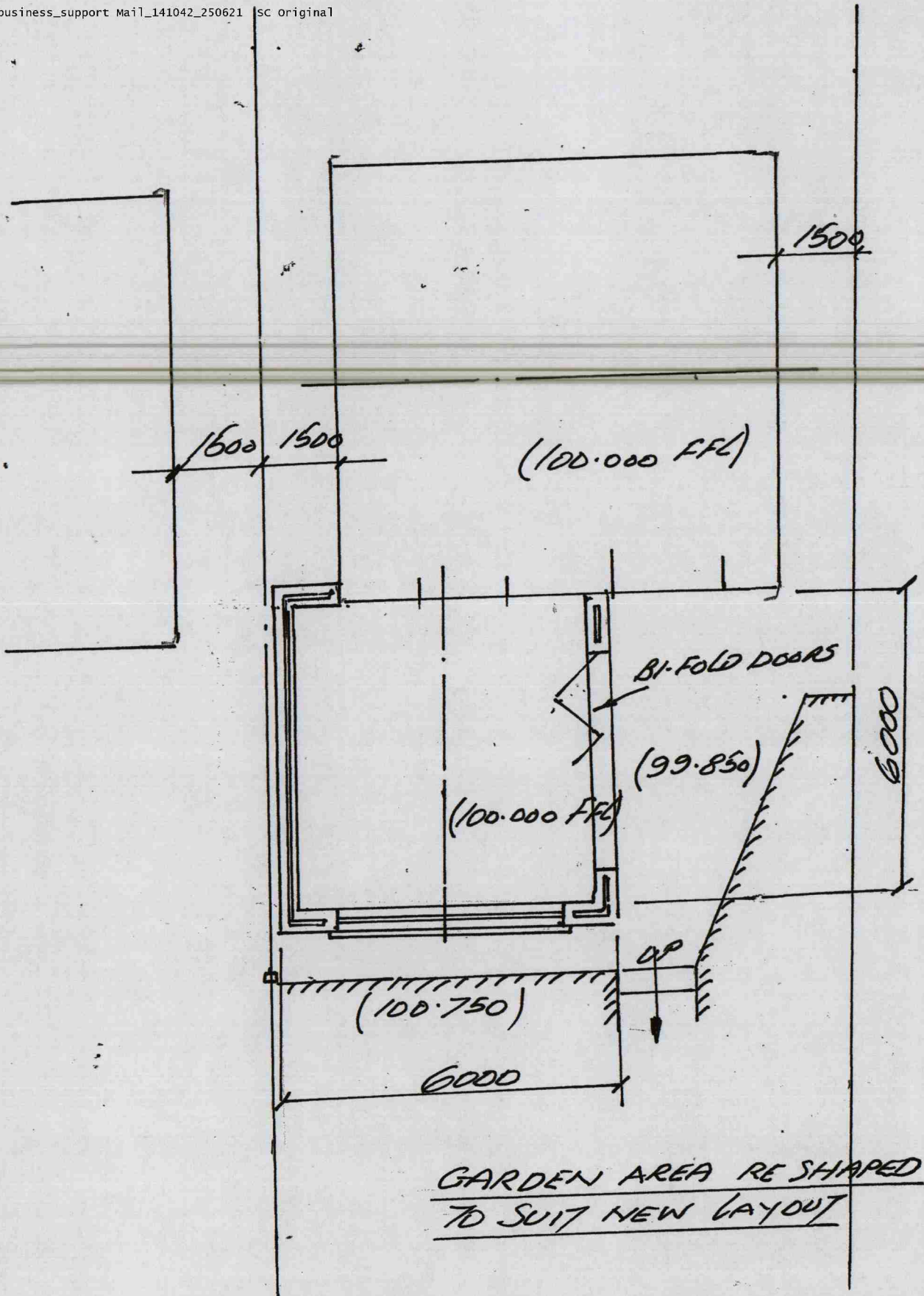
PLAN ON PROPOSED GROUND FLOOR (1:100) (SCALE 1:100)
