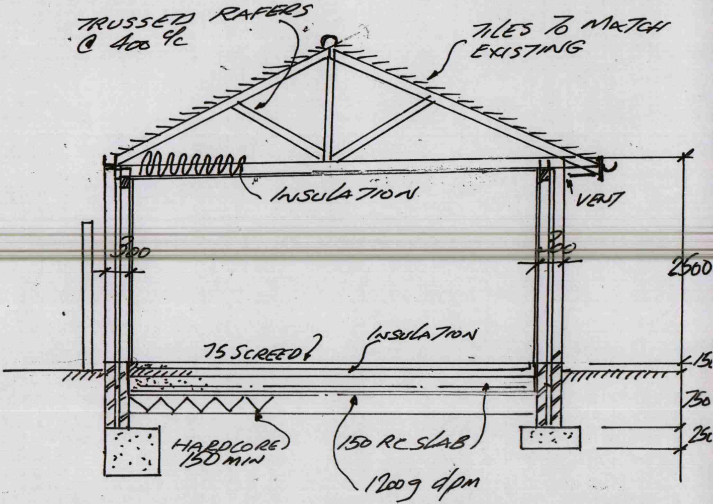
TYPICAL CROSS SECTION (1:50)
