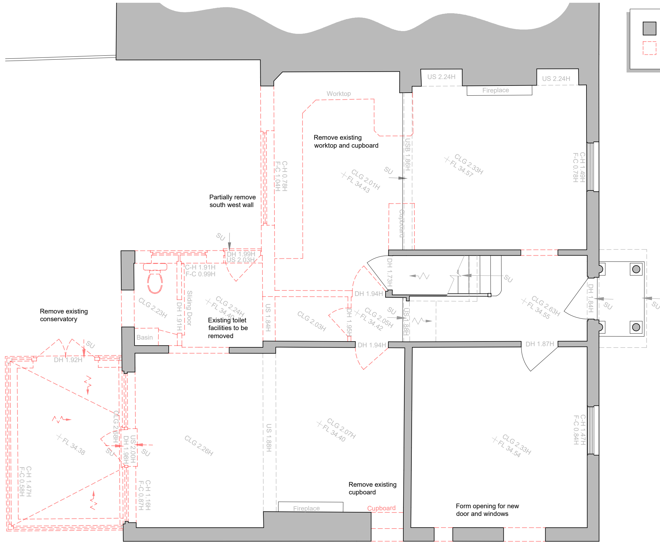
Proposed Ground Floor Plan Scale 1:50 @ A3
