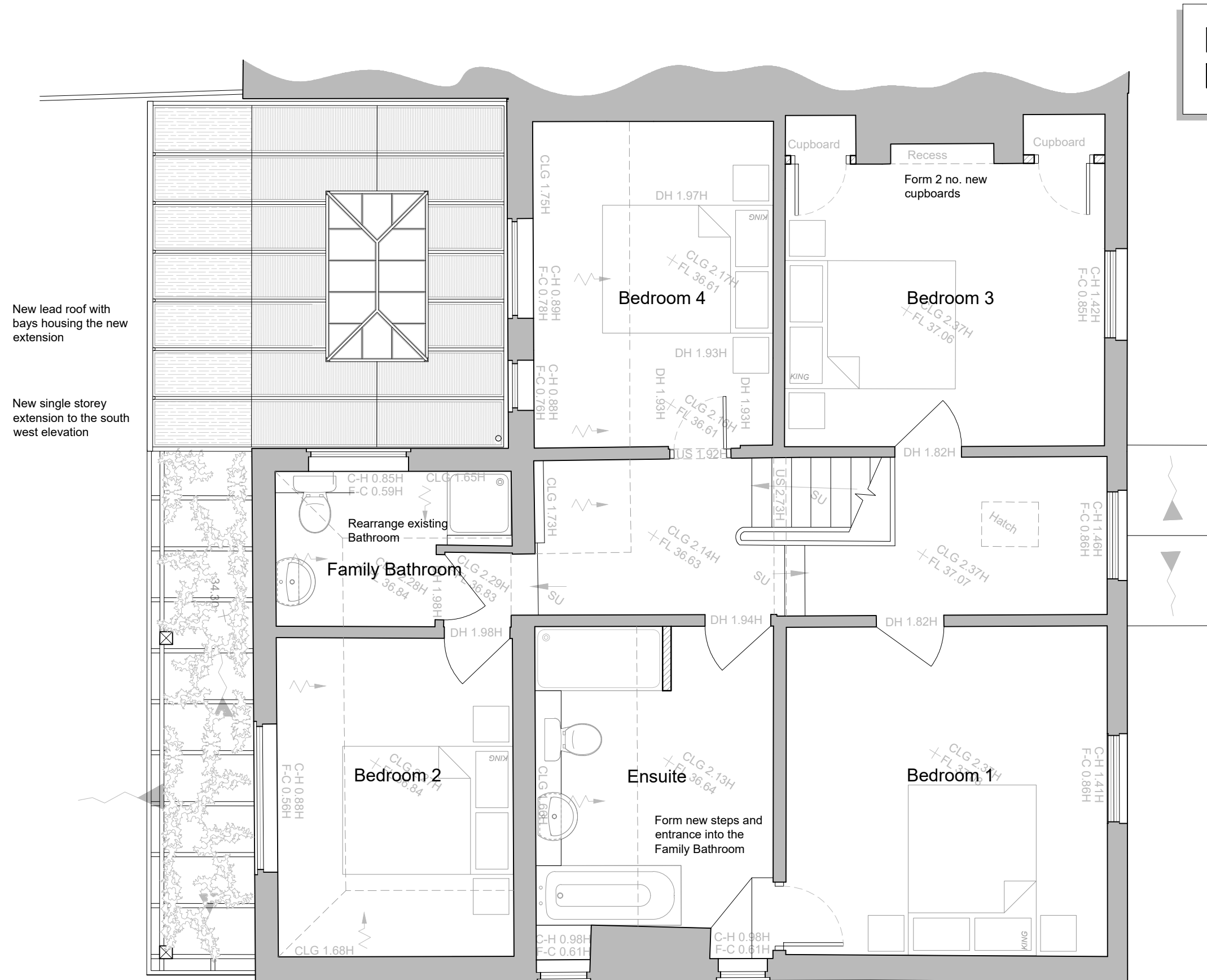
Proposed First Floor Plan Scale 1:50 @ A3
