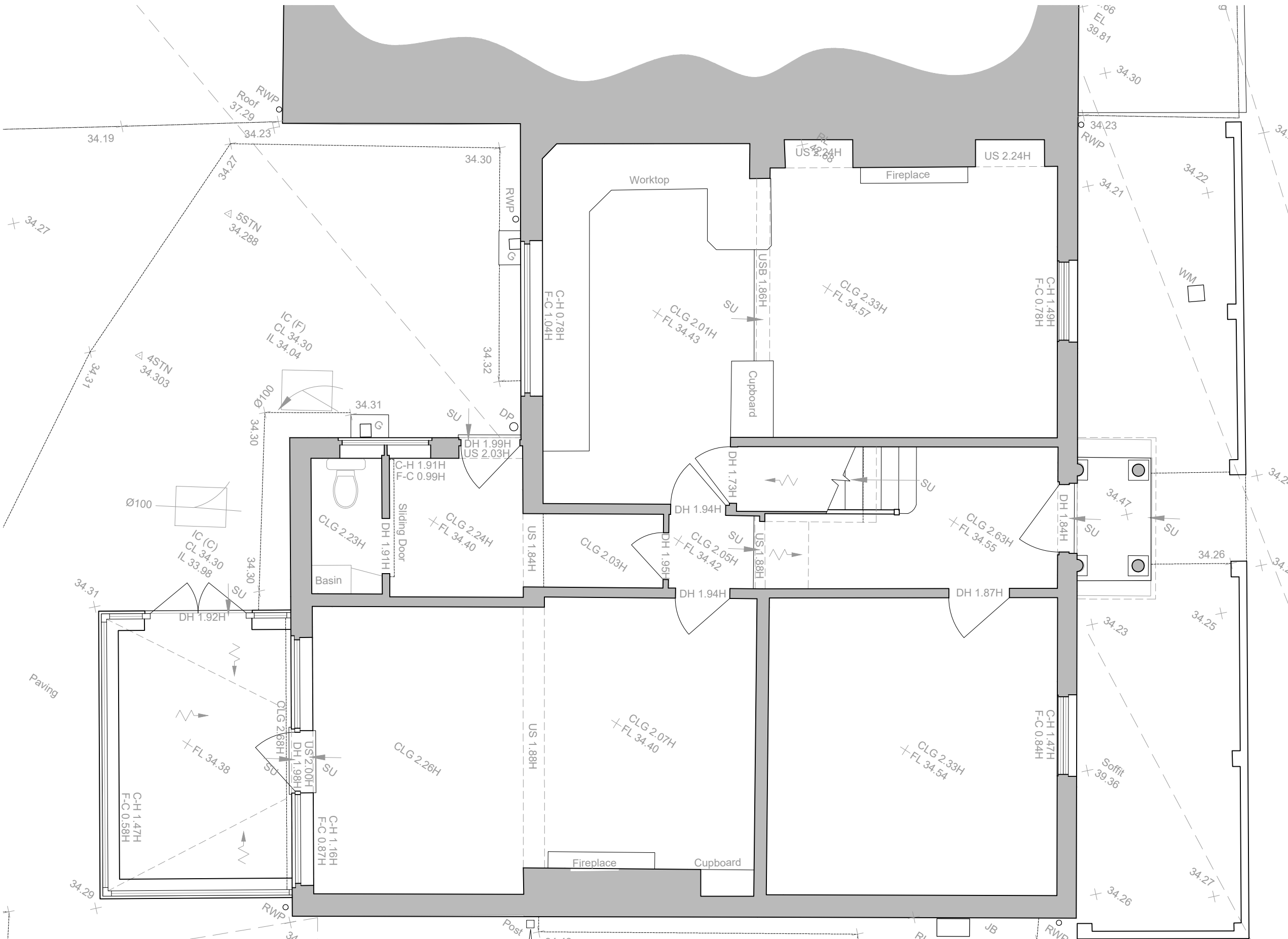
Existing Ground Floor Plan Scale 1:50 @ A3
