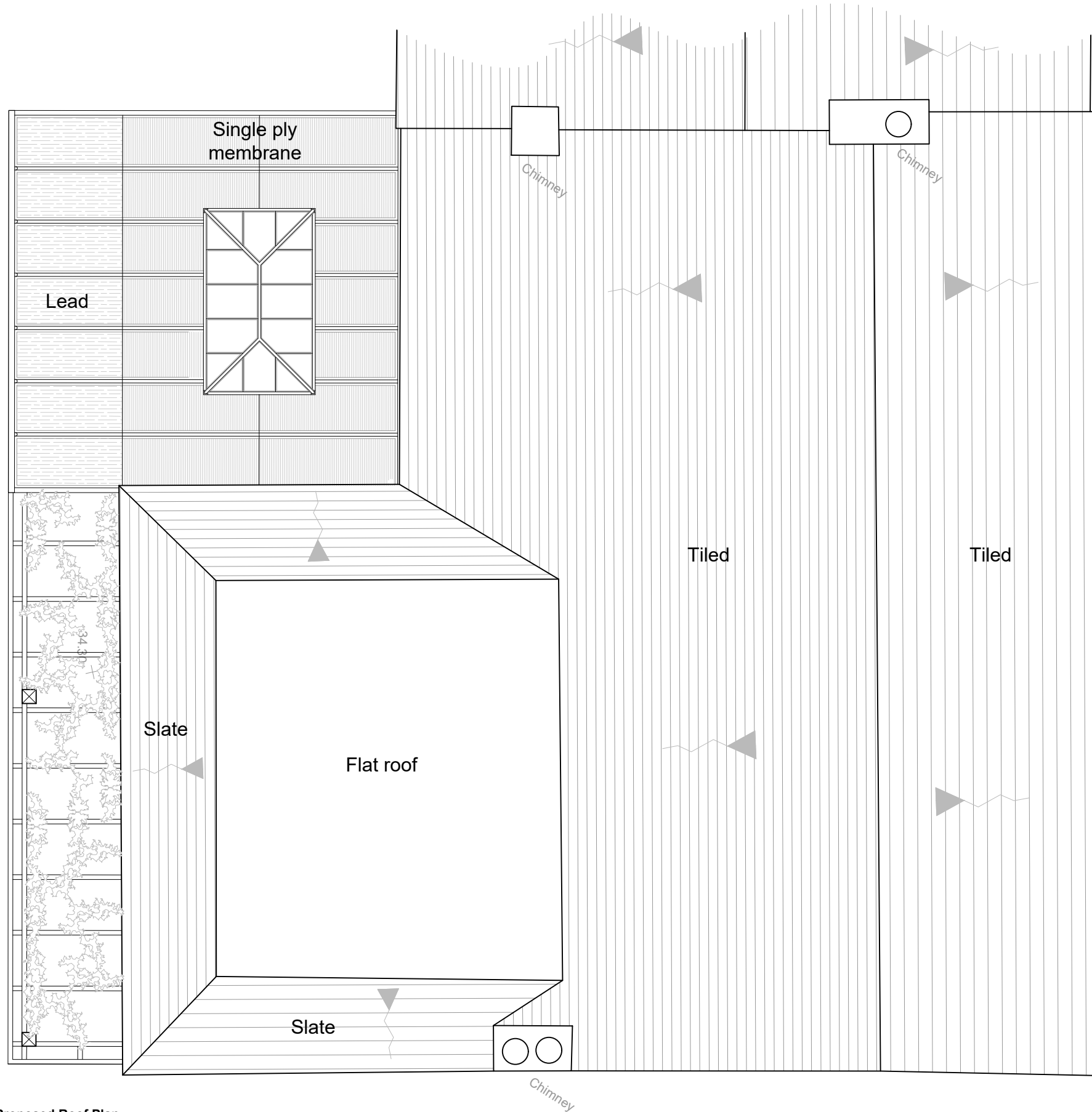
Proposed Roof Plan Scale 1:50 @ A3
