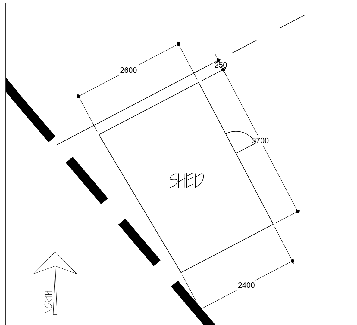
FLOOR PLAN - 1:50
