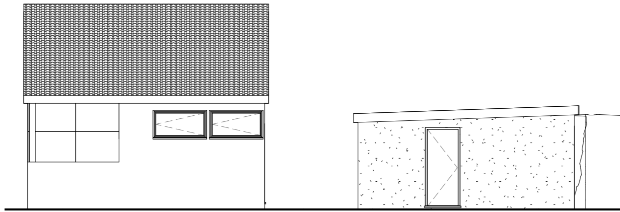
1 East Elevation 1 : 100
