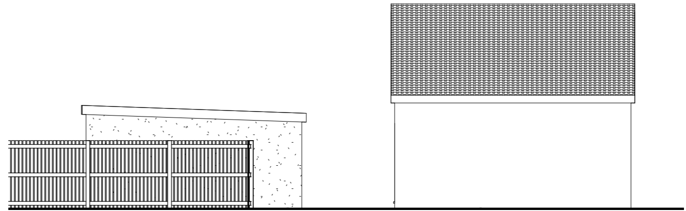
4 West Elevation 1 : 100
