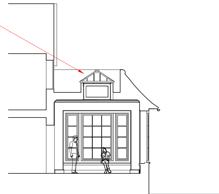
02. Proposed Section 1:100
