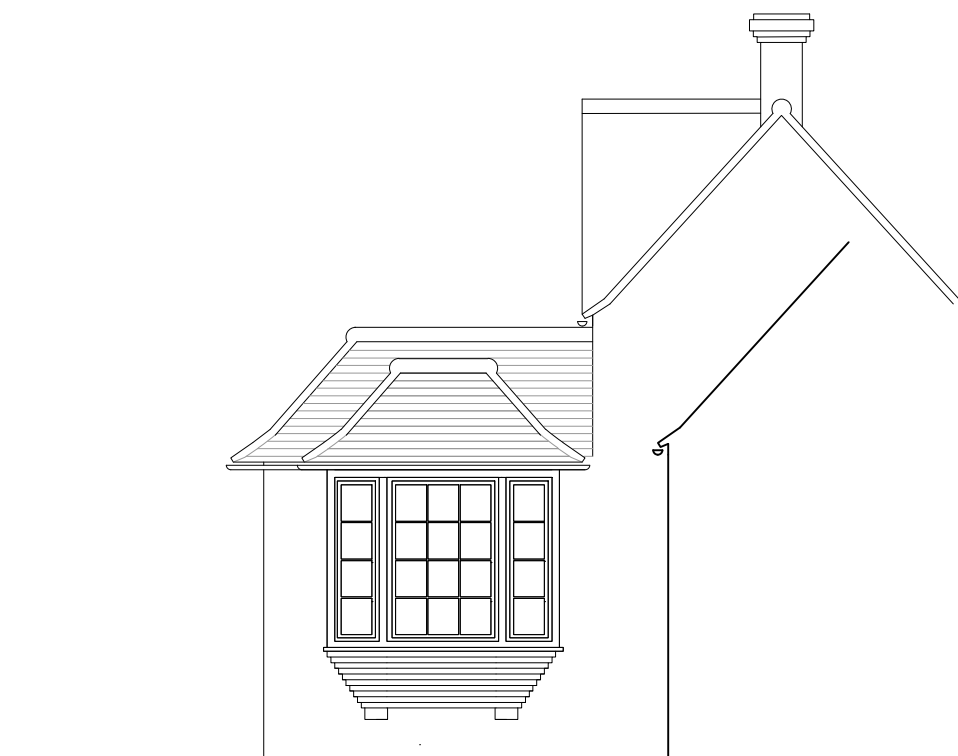
03. Proposed West Elevation 1:100
