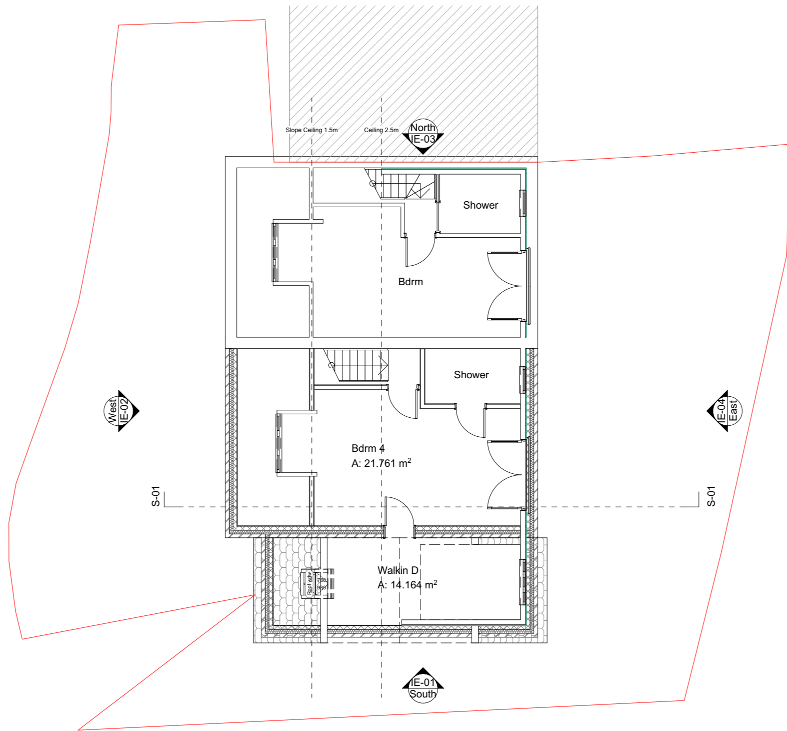
Proposed 2nd Flr 1:100
