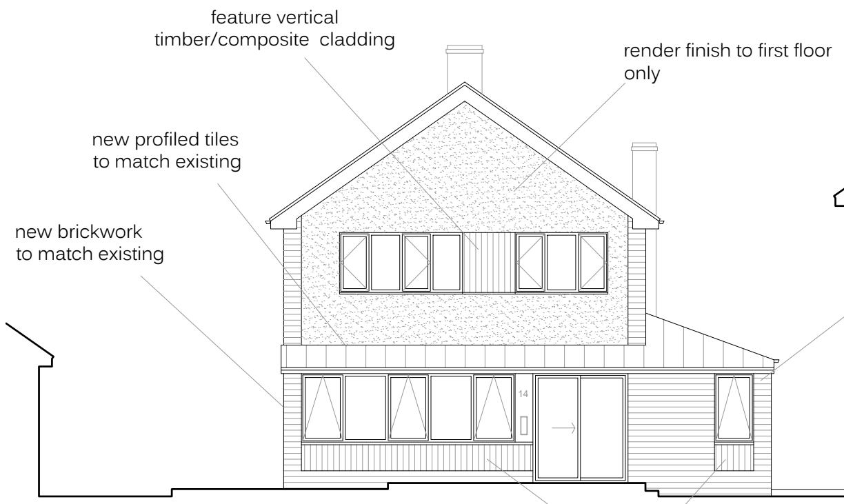
1. front elevation
