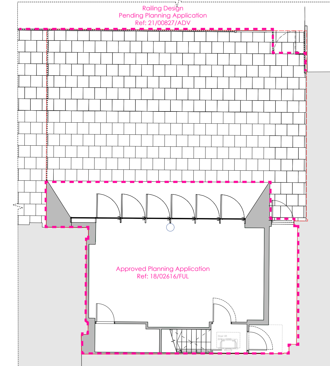
Previously Approved Ground Floor Plan - Ref: 18/02616/FUL
