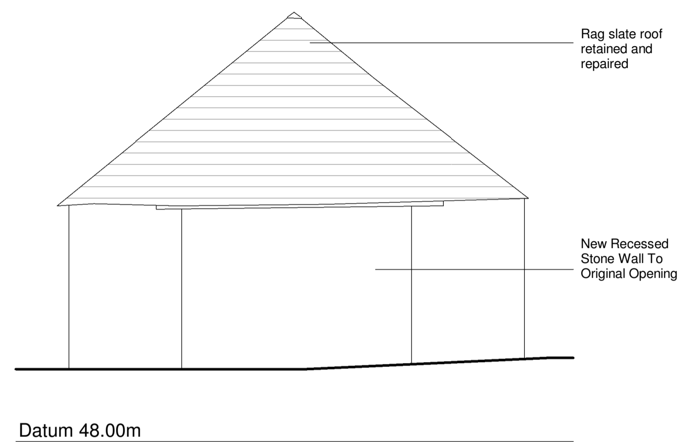
North Elevation
