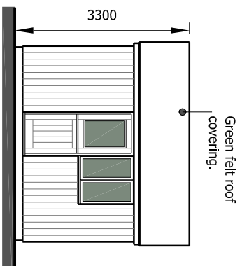
Proposed Front Elevation 1:100
