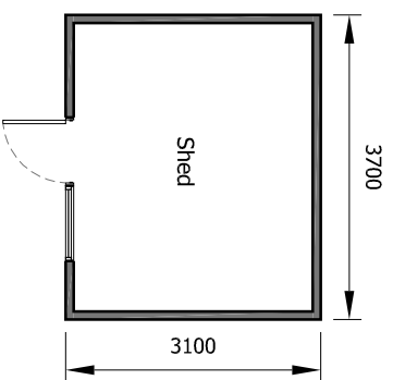
Proposed Floor Plan 1:100
