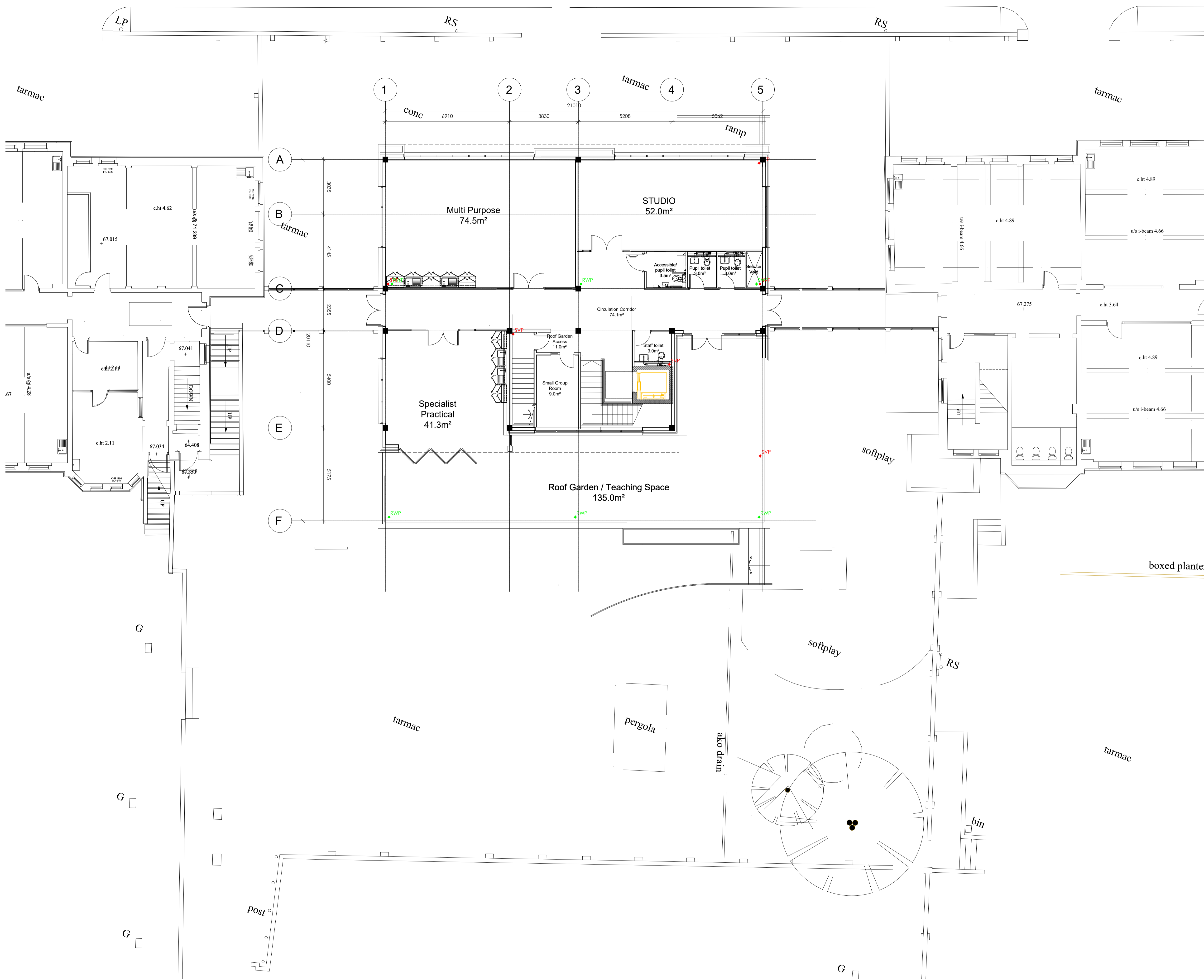
PROPOSED FIRST FLOOR PLAN Scale: 1:100
