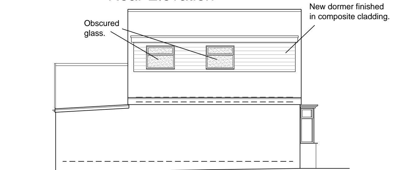
Rear Elevation
