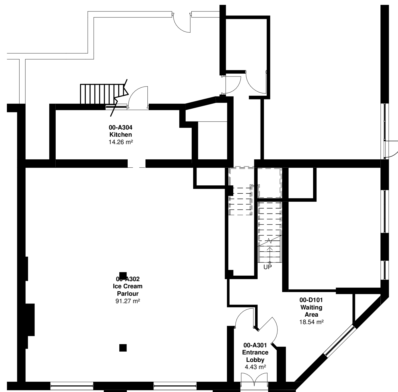
1 10-00_GA Plan as Existing - Level 00 1:100
