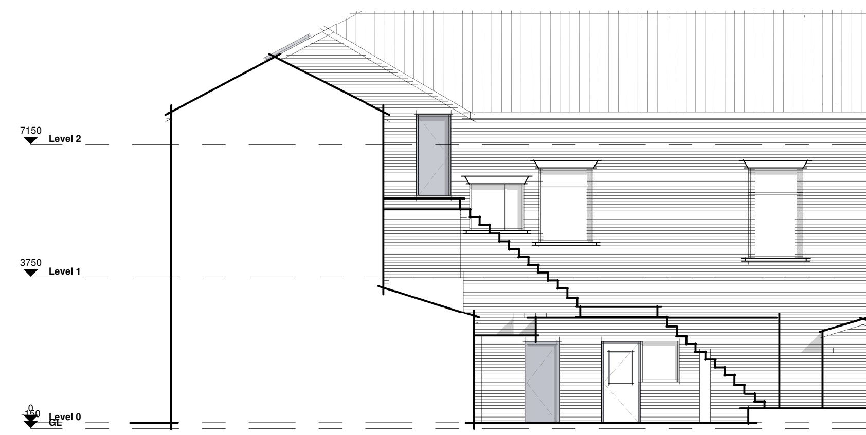
6 1103 Existing Elevation 3 1:100
