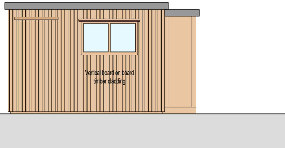
EAST ELEVATION
