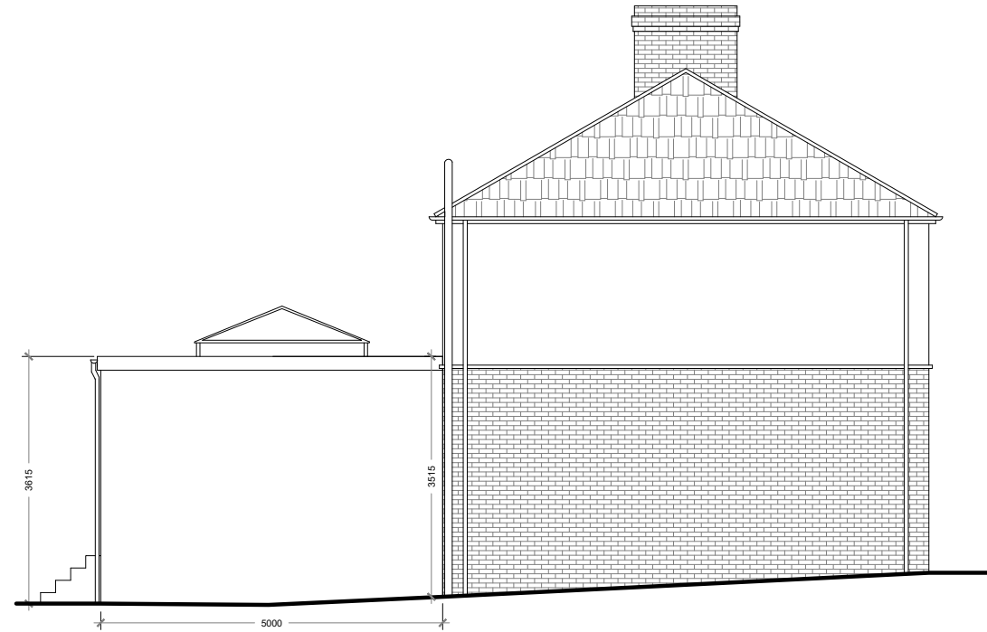
Side Elevation
