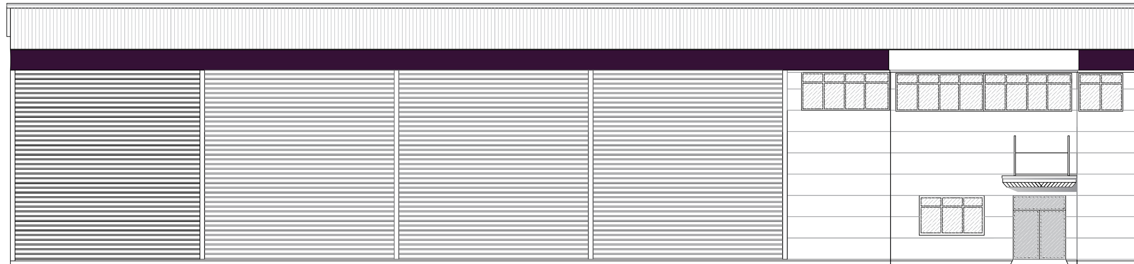
South West Elevation 1:100 @ A1
