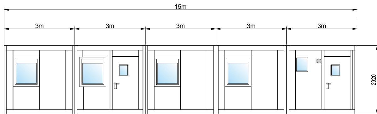
FRONT ELEVATION
