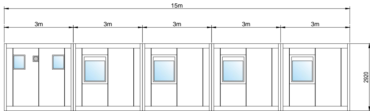
REAR ELEVATION
