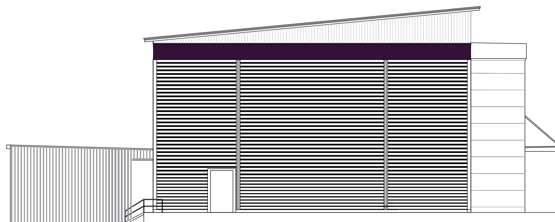
North West Elevation 1:100 @ A1
