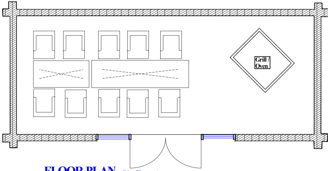
FLOOR PLAN (No Change)
