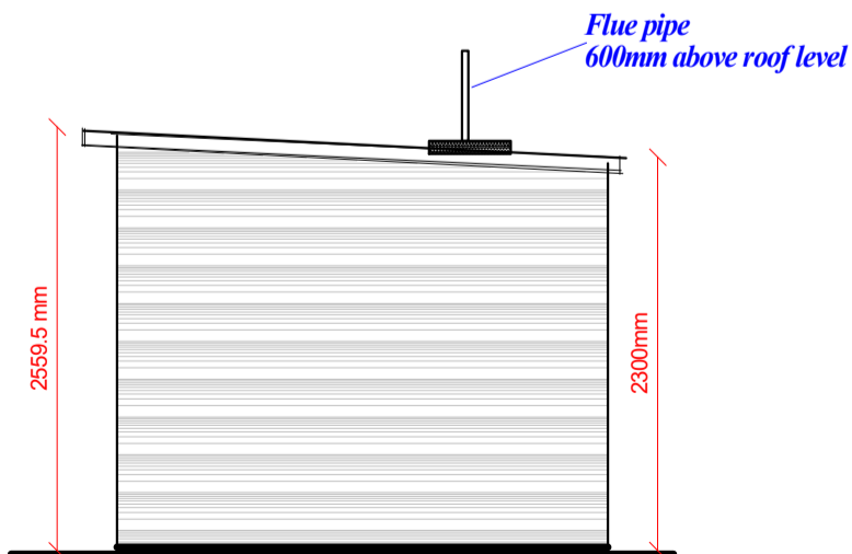
RIGHT SIDE ELEVATION (No Change)
