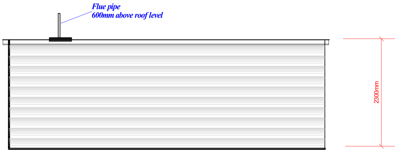
REAR ELEVATION
