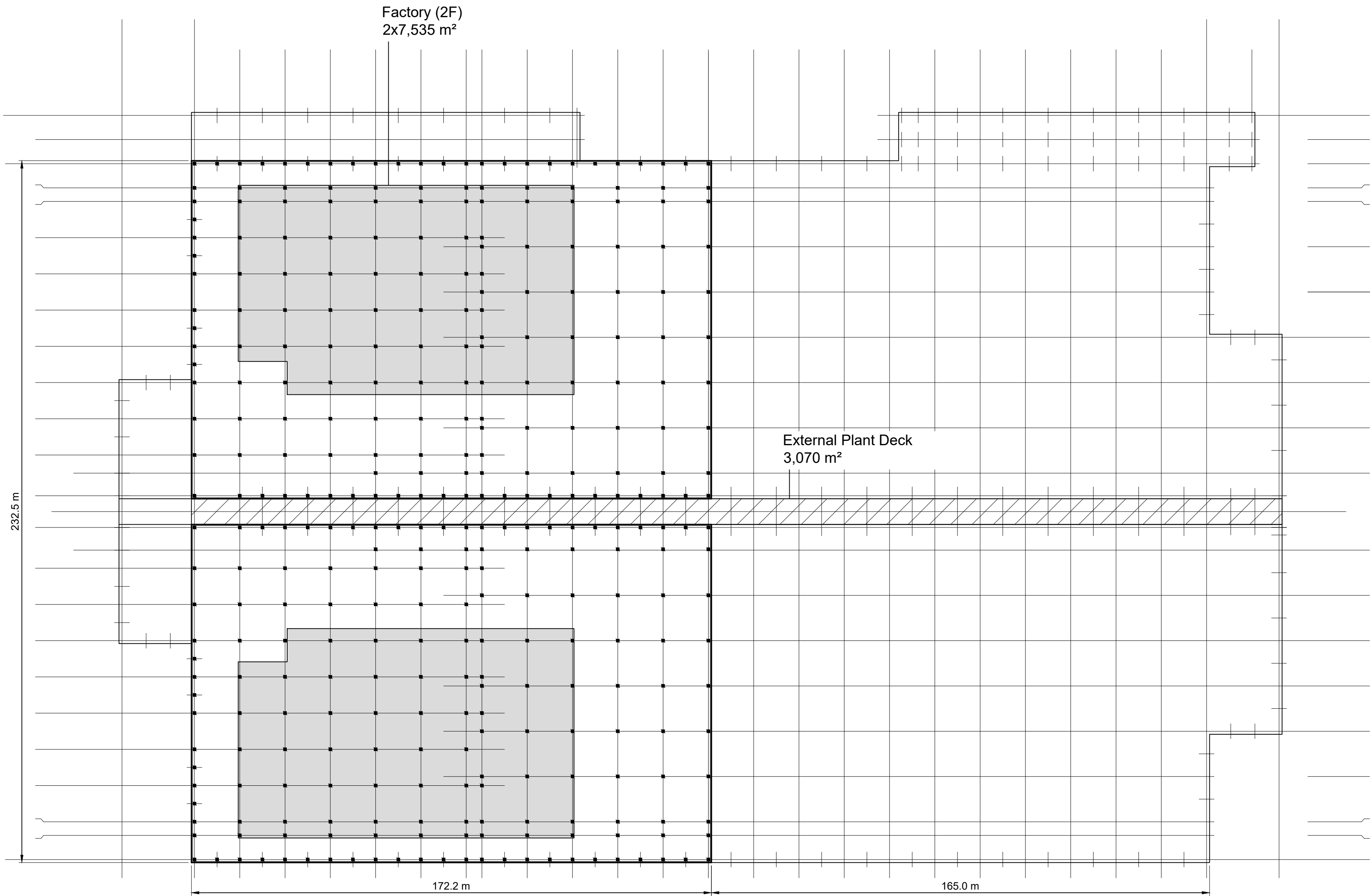
First Floor Plan - Process (2F)
