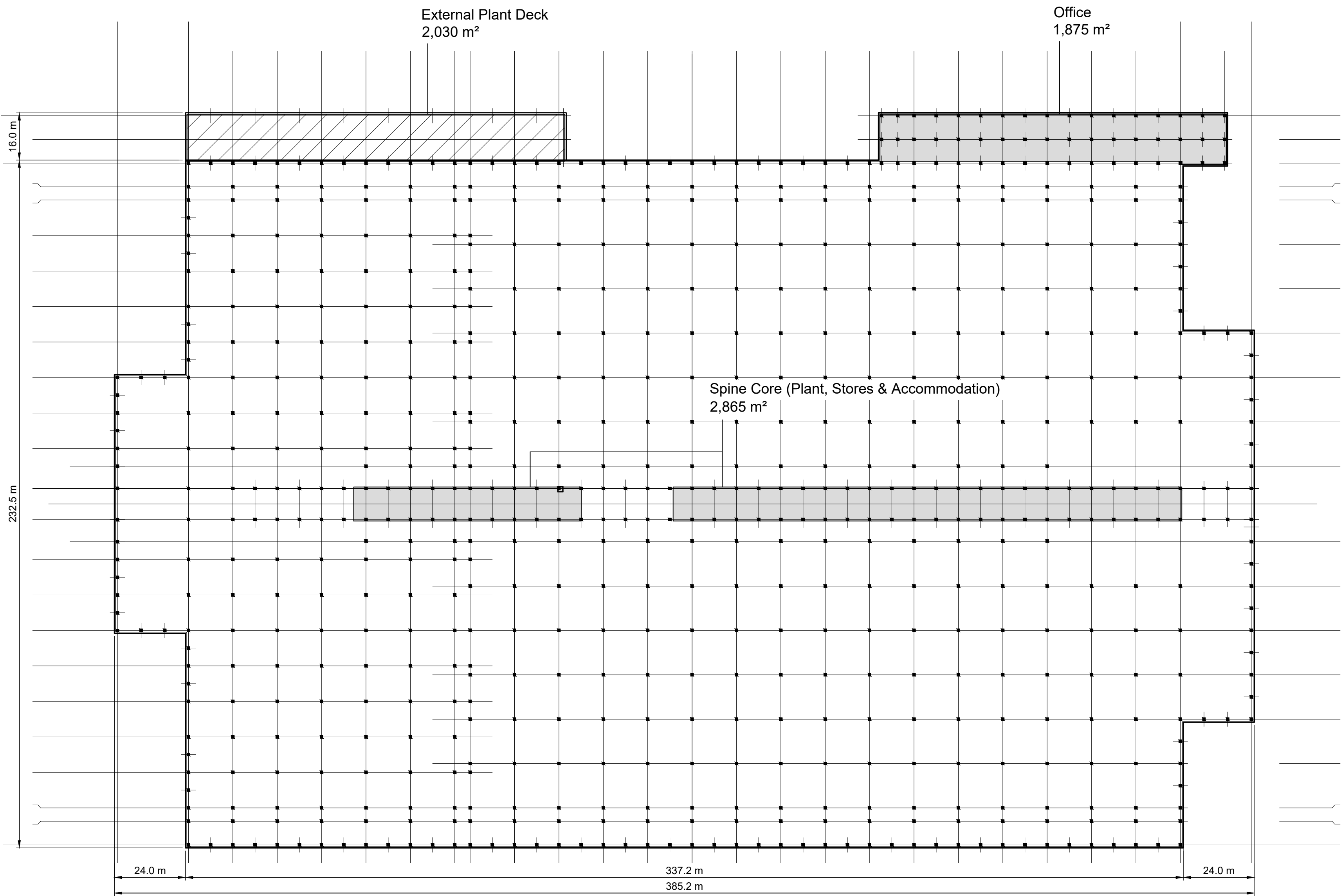
First Floor Plan - Admin / Offices / Plant Deck (2F)
