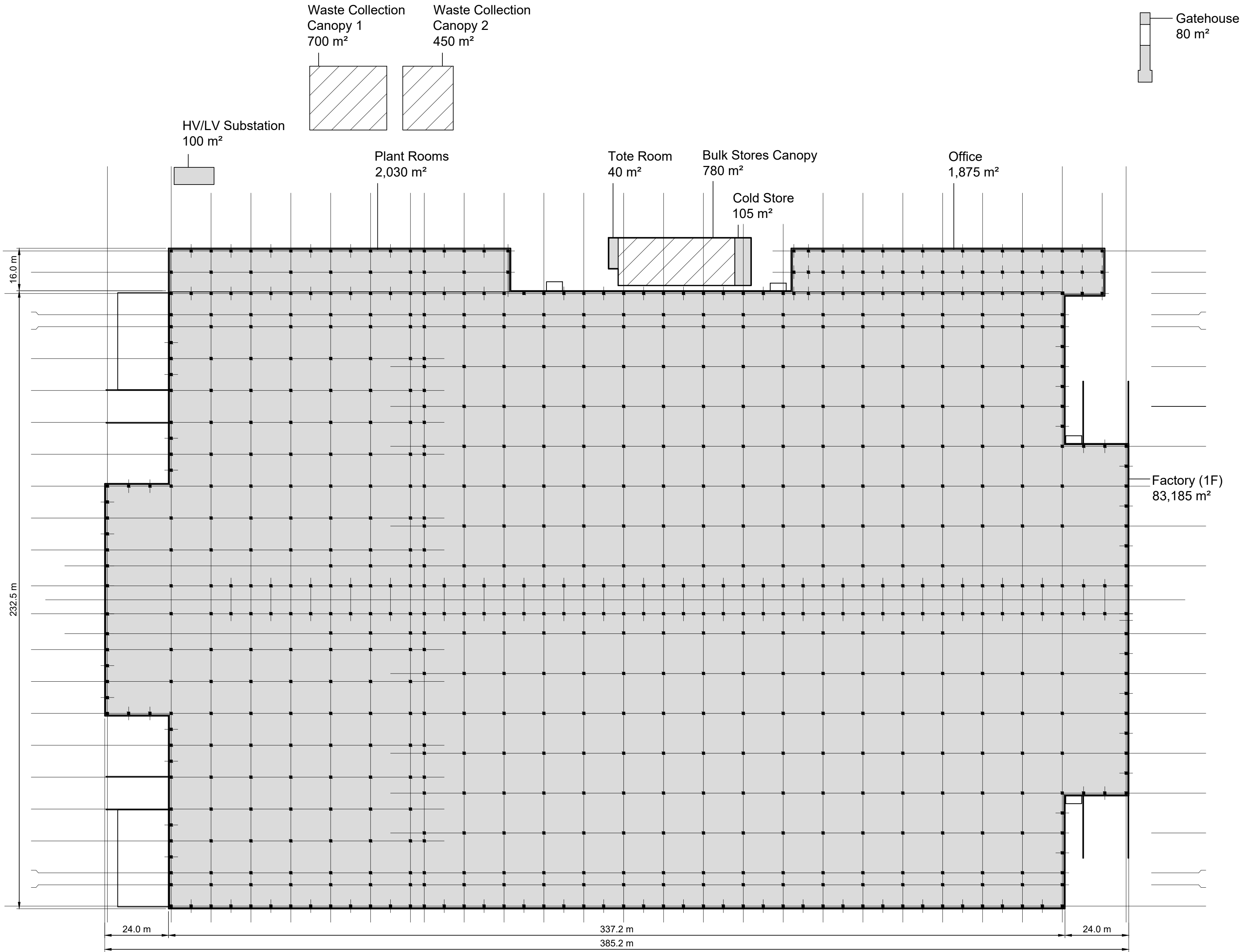
Ground Floor Plan (1F)
