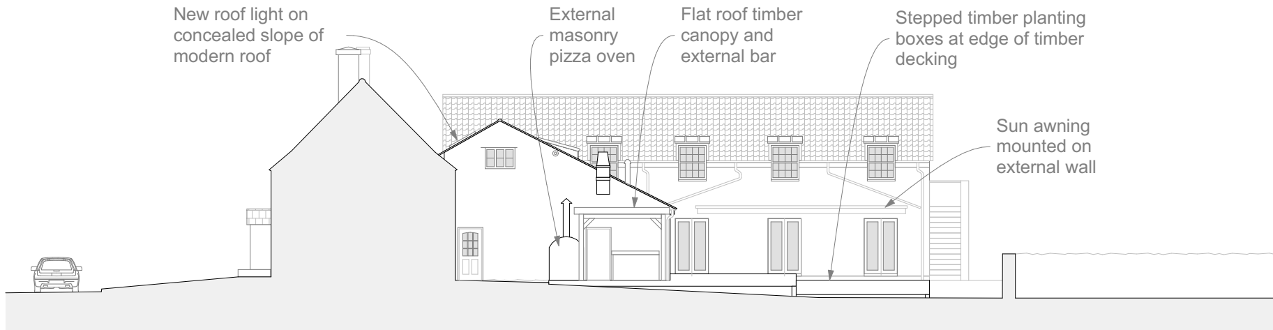
SOUTH EAST (GARDEN) ELEVATION
