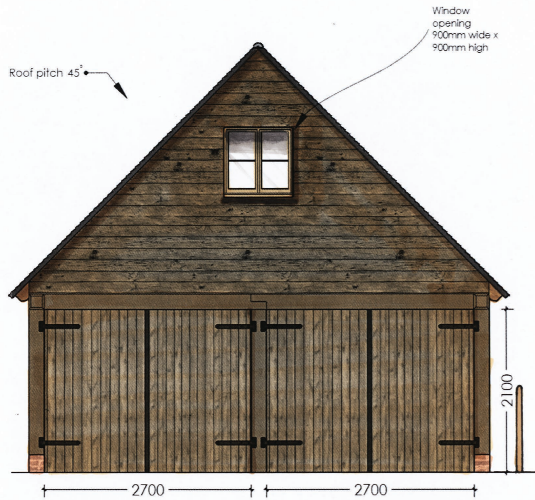
Front Elevation North
