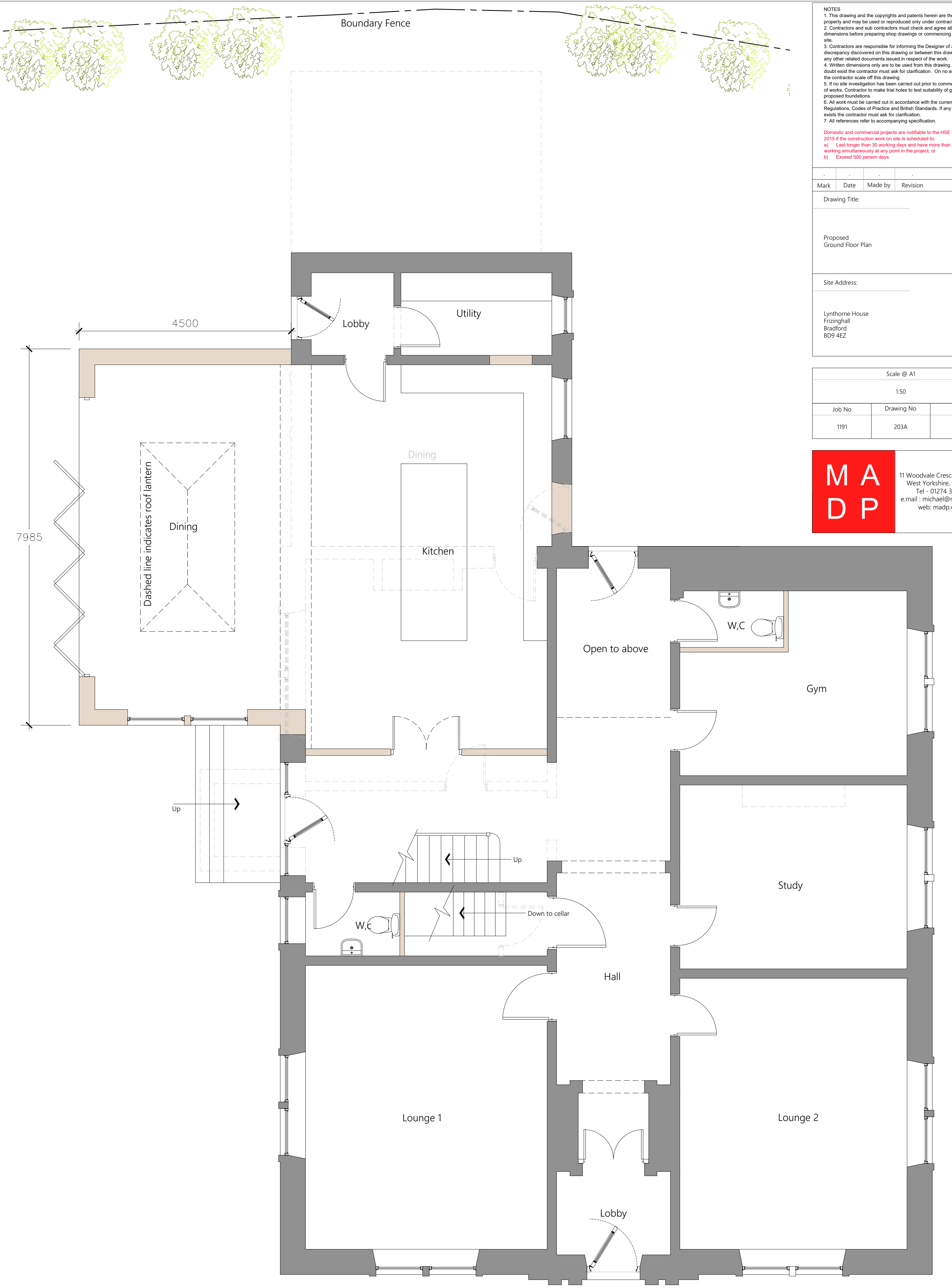
Ground Floor Plan 1:50
