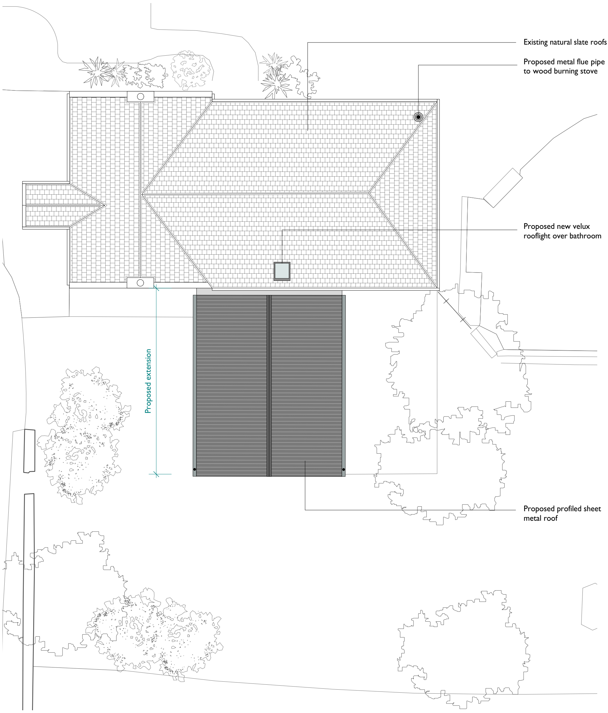
Proposed Roof Plan Scale: 1:100
