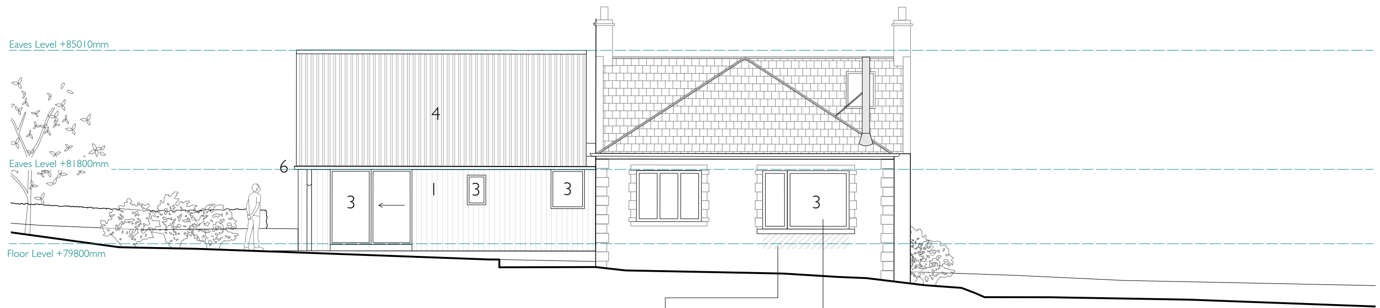
Existing East Elevation Scale: 1:100
