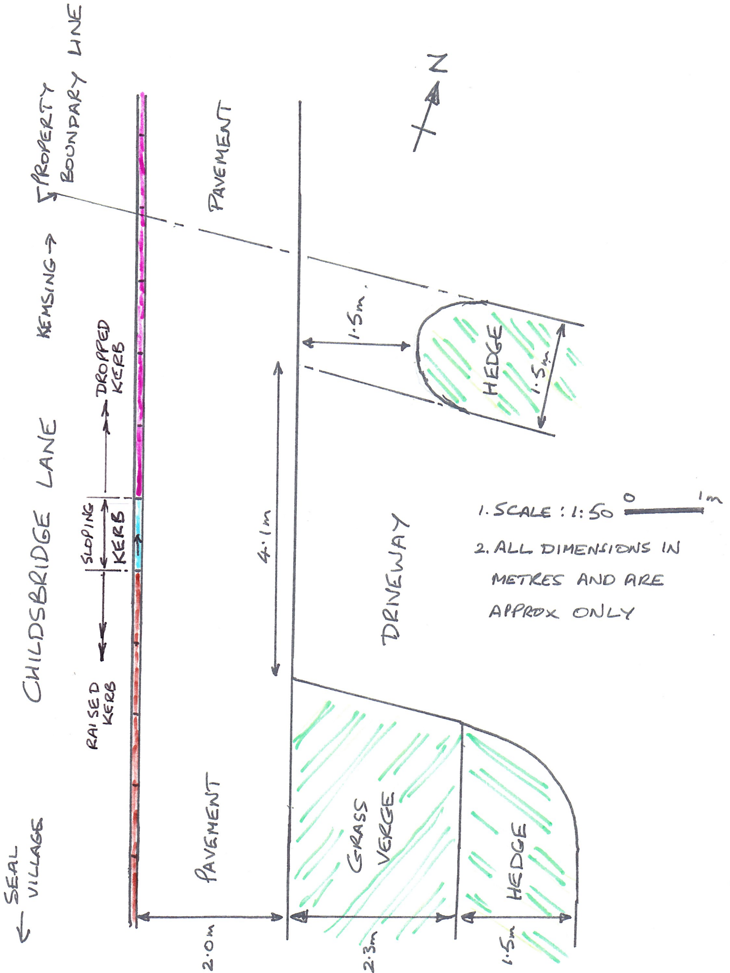
FIGURE 4 EXISTING LAYOUT
