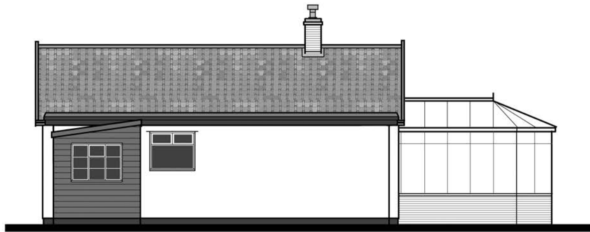
:: Rear (West) :: Existing :: 1:100 ::
