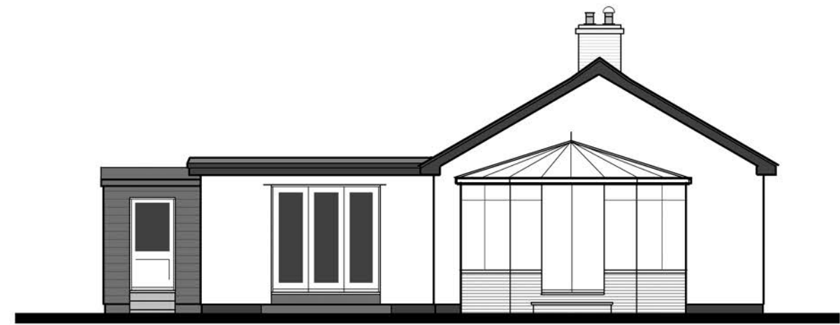
:: Side (South) :: Existing :: 1:100 ::
