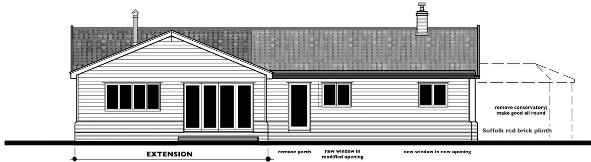
:: Rear (West) :: Proposed :: 1:100 ::
