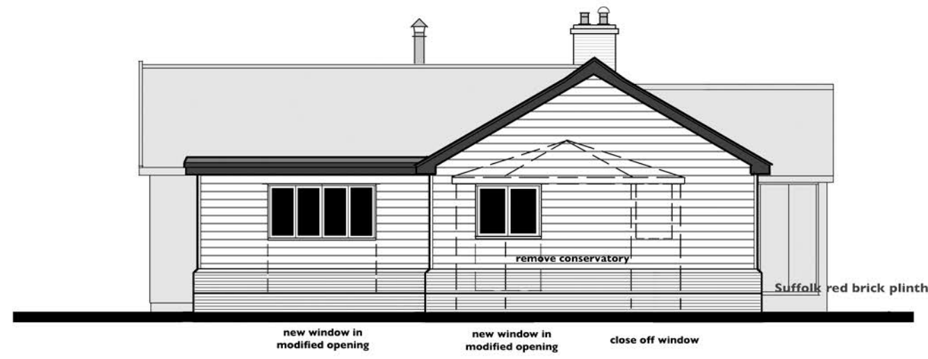
:: Side (South) :: Proposed :: 1:100 ::
